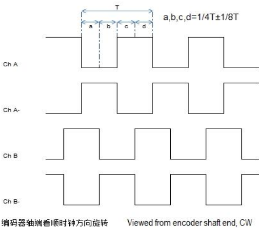
编码器轴端看顺时针方向旋转 Viewed from encoder shaft end, CW
